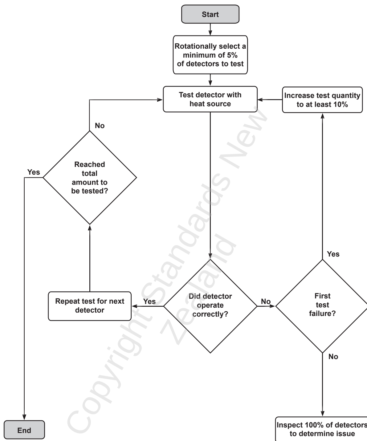
Figure 5 – Heat detector annual sample testing flow chart
