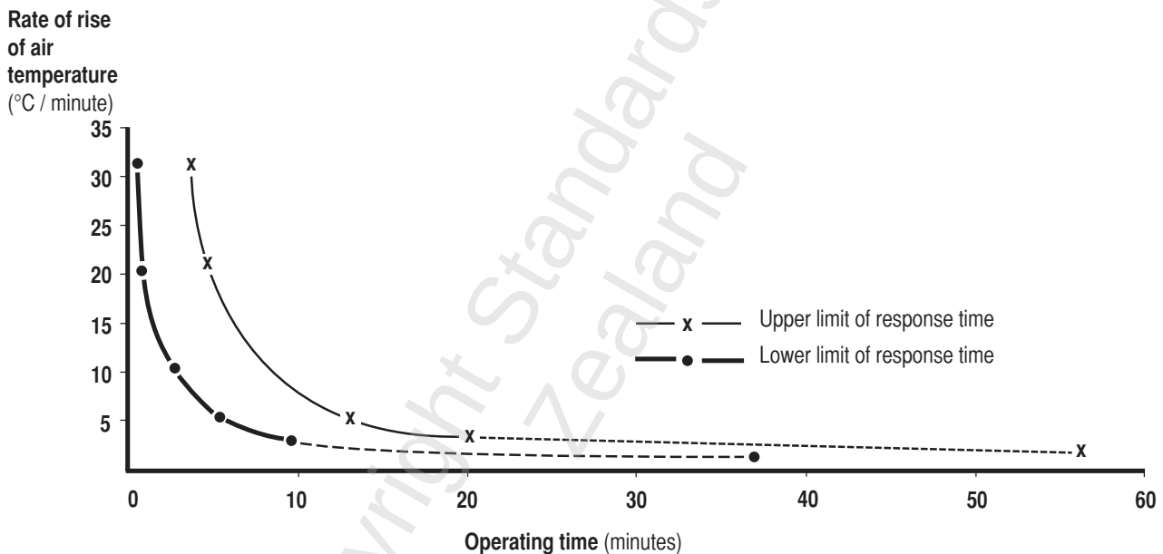
Figure E3 – Rate-of-rise heat-actuated fire detectors
