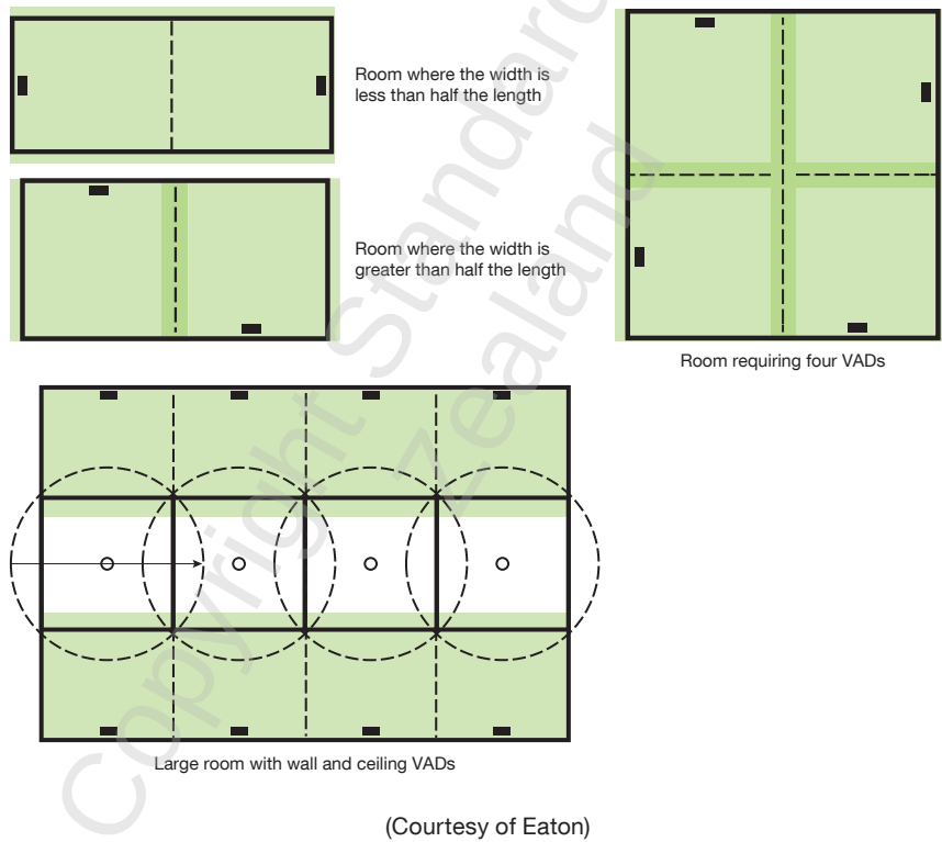
Figure L4 – VAD location examples
