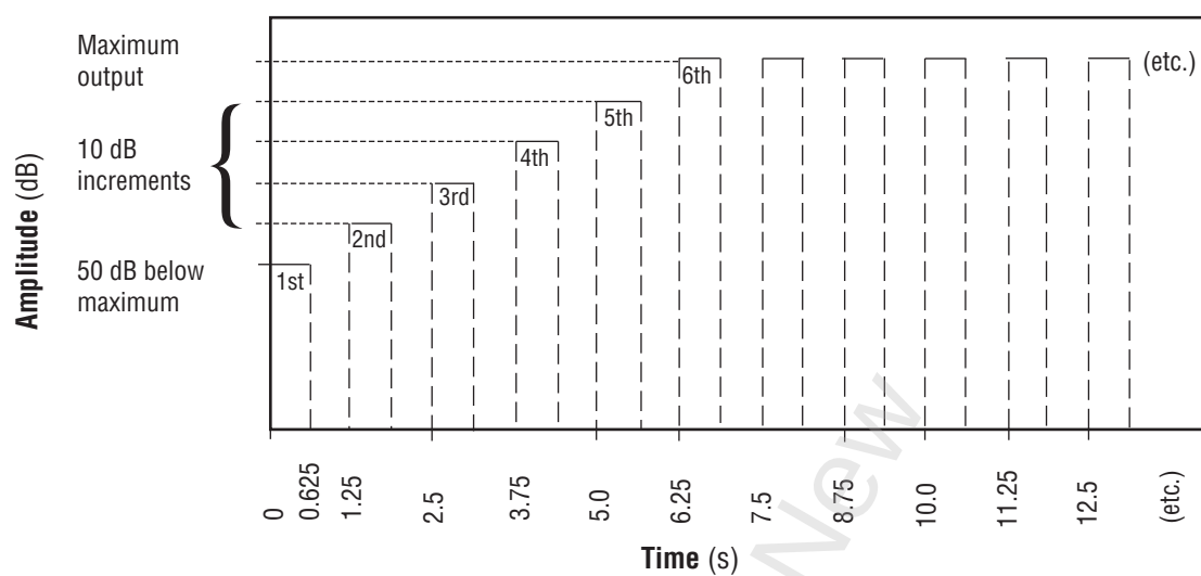
Figure G2 – Alert signal
