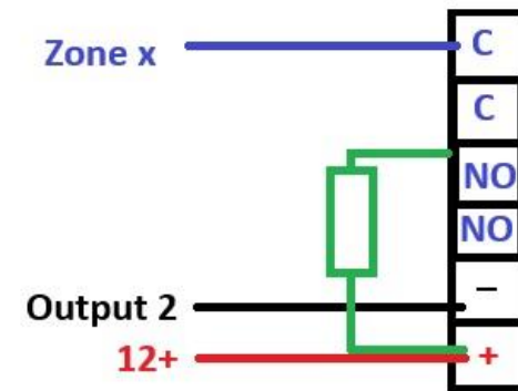
Original wiring config to old Bosch 880/408/448 etc
